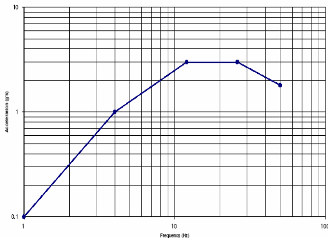
ASTM Truck Assurance Level 1 Calculated Vertical Performance 1000 lbs. Payload
