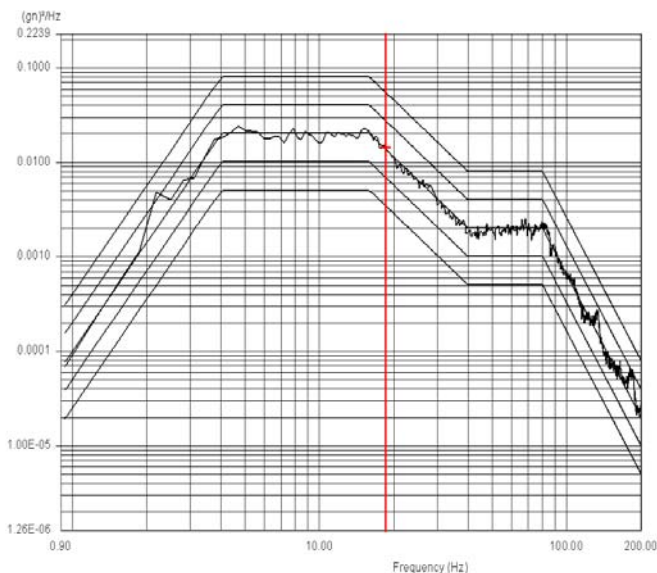
ASTM Truck Assurance Level 1 Calculated Vertical Performance 1000 lbs. Payload
